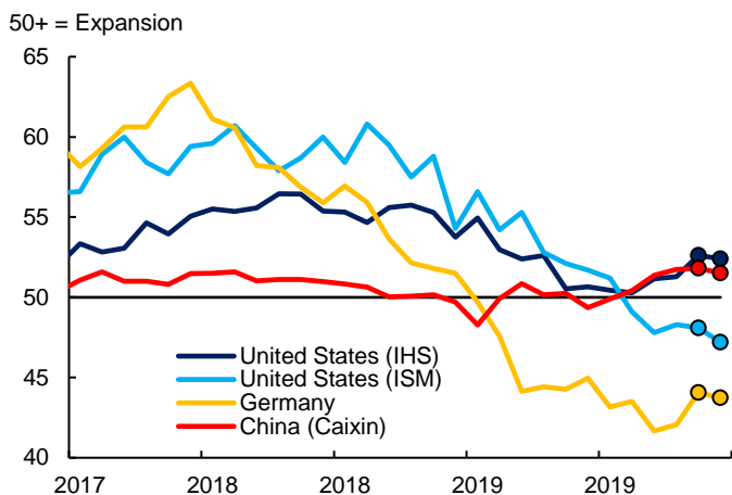
Figure 3: Manufacturing PMIs
